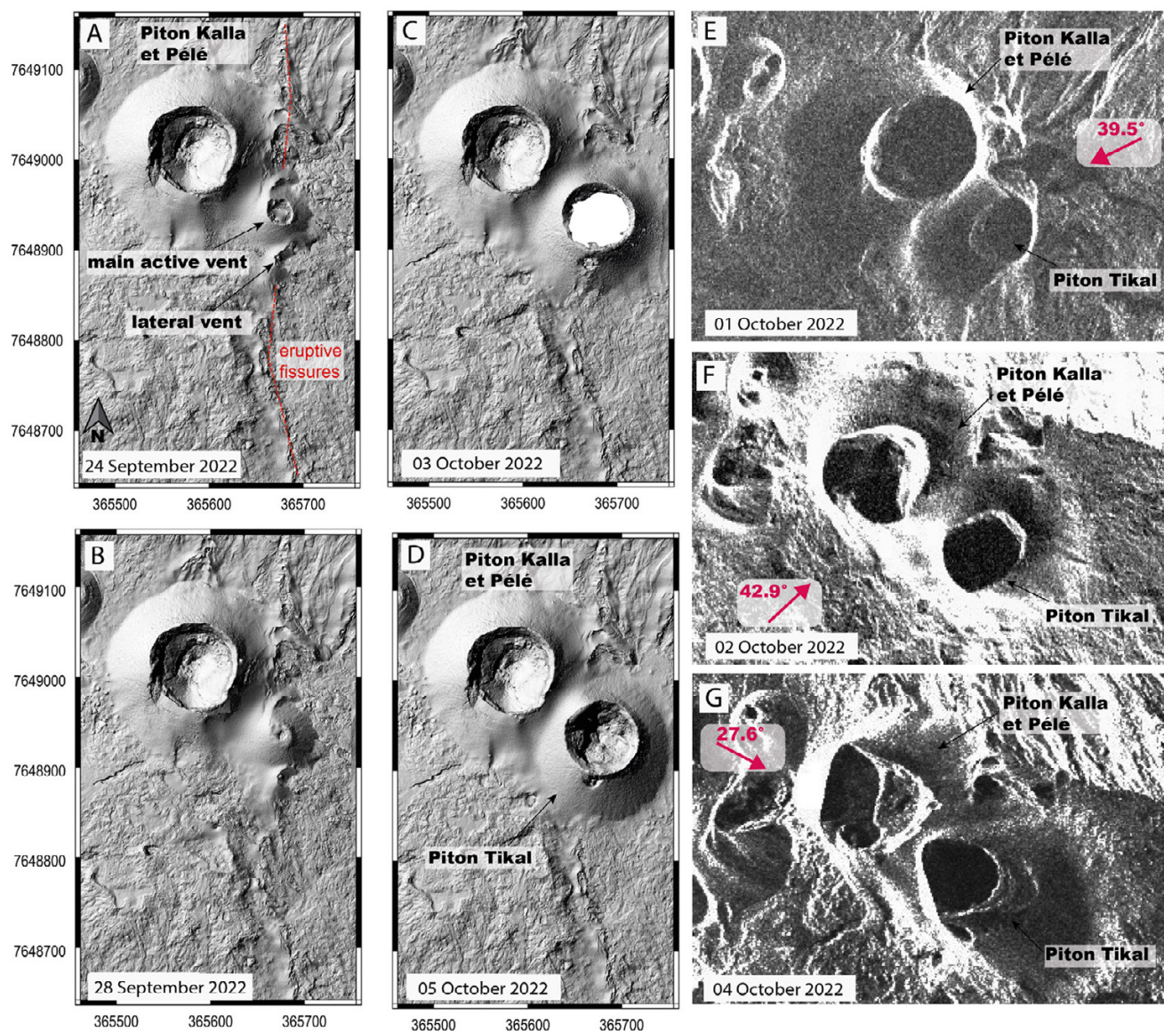
Figure 5: Evolution of the eruptive cone morphology. [A–D] Hillshade DSM (north toward the top) showing the eruptive vent (named Piton Tikal at the end of the eruption) growing to the east of an old cone Piton Kalla et Pélé . Images were obtained by aerial SfM photogrammetry taken via ULM on 24 September and 5 October and via UAS on 28 September and 3 October. On the image of 03 October, topography inside the crater of Piton Tikal could not be obtained. [E–G] Capella SAR images taken on 01, 02 and 04 October. These images are SLC images containing geometrical distortions. Viewing direction and incidence angle with respect to vertical are indicated by the pink arrow. Images are rotated north-up to facilitate interpretation. They are roughly at the same scale as the DSM. The dates of acquisition are indicated on the images.
