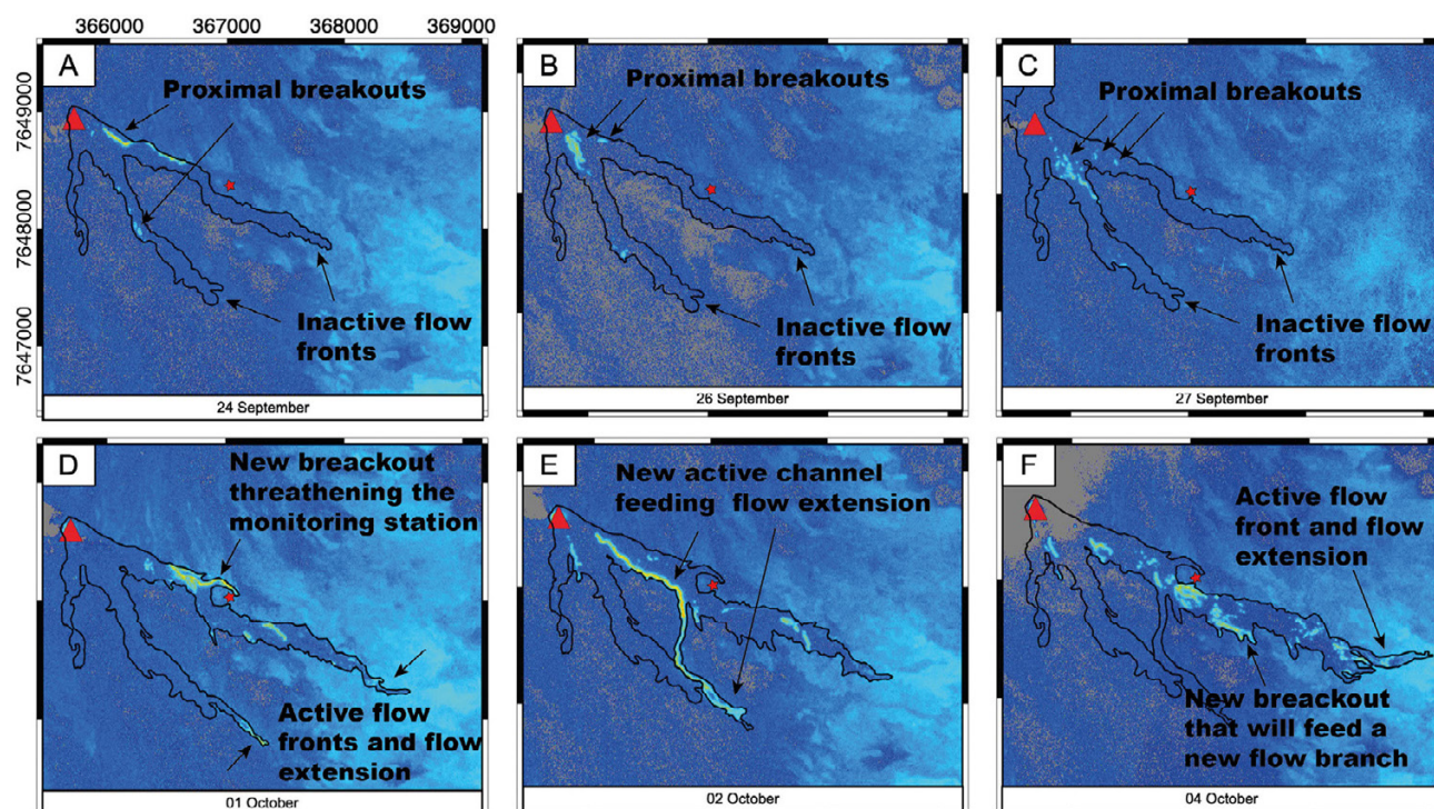
Figure 7: Images from PlanetScope filtered with red edge triangular vegetation index (RTVI) showing the active parts of the flow through emplacement over the eruption. The red triangle represents the main vent. The red star indicates the location of the monitoring station. Indices color scale (cold to warm) reflect thermal radiation intensity emitted by active lava flow. [A–C] are acquired during the phase of low effusion rate between 20 to 29 September while [D–F] are acquired during the phase of higher effusion rate between 29 September to 05 October.
