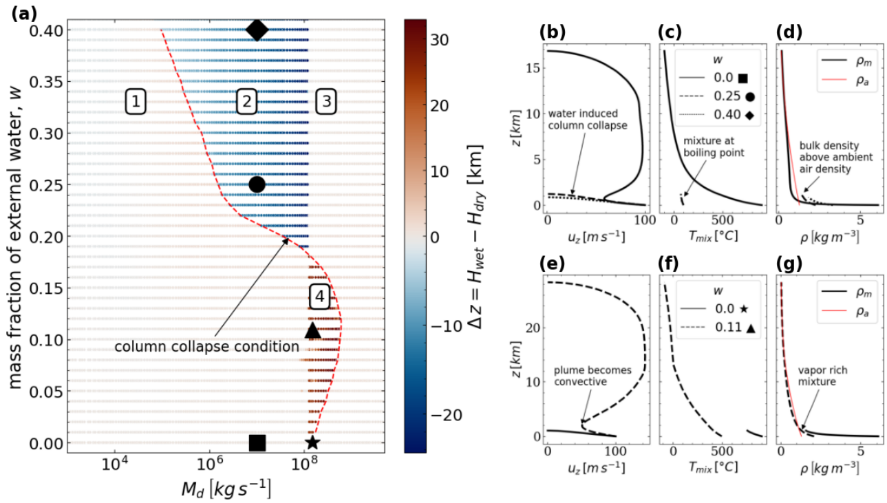
Figure 3: (a) Effect of external water, w , on column height difference relative to the dry case ( \Delta z , km) for various initial mass eruption rates ( M_d , \text{kg s}^{-1} ) and for the initial conditions corresponding to Figure 2e. The numbers in the squares represent the four collapse-response regimes describing how external water modifies the column collapse condition. The column collapse condition marks the point at which buoyant plumes cease to form. Black symbols denote the initial conditions of the runs shown in panels (b–g): the triangle corresponds to regime 4 (panels e–g); the circle and diamond correspond to regime 2 (panels b–c); and the square and star represent the no-water equivalents of regimes 2 and 4. Panels (b–g) show results from individual Plumeria simulations with initial mass eruption rate values of \sim 10^7 and \sim 10^8 \text{ kg s}^{-1} in panels (b–d) and (e–g), respectively. The ambient air density profile is shown for reference in panels (d) and (g).
