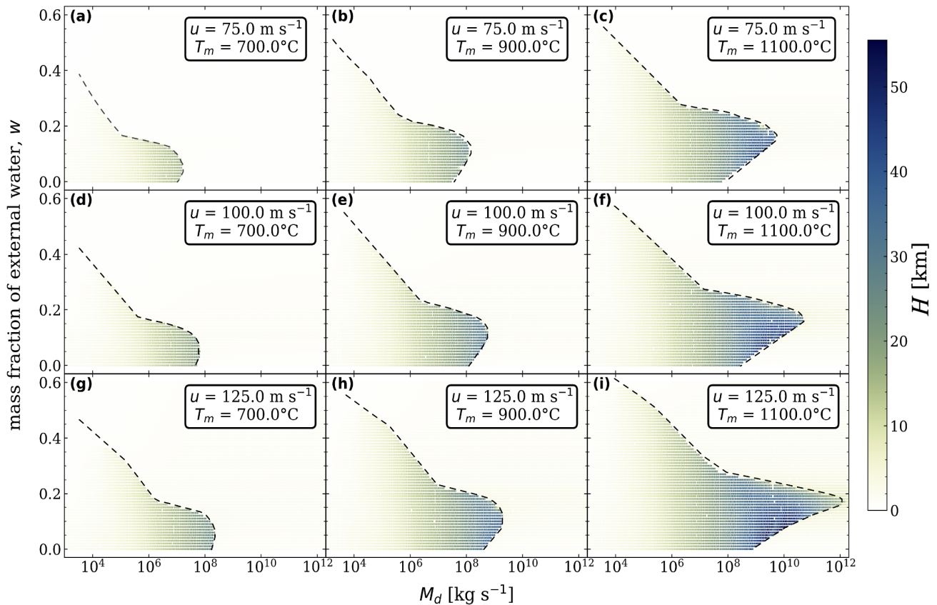
Figure 2: Plumeria results for maximum column height ( H , km) as a function of mass fraction of external water ( w ) and mass eruption rate ( M_d , \text{kg s}^{-1} ). Panels (a-i) show the results of the varying vent exit velocities ( u ) and initial magma temperatures ( T_m ) (see panel annotations). The black dashed lines identify a distinct boundary indicating a mass flux threshold at which buoyant plumes cease to form under varying external water contents (column collapse condition). The columns' initial magma temperature and vent exit velocity affect the column collapse condition's location.
